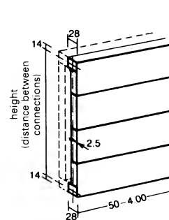
6 Section through a flat panel radiator
